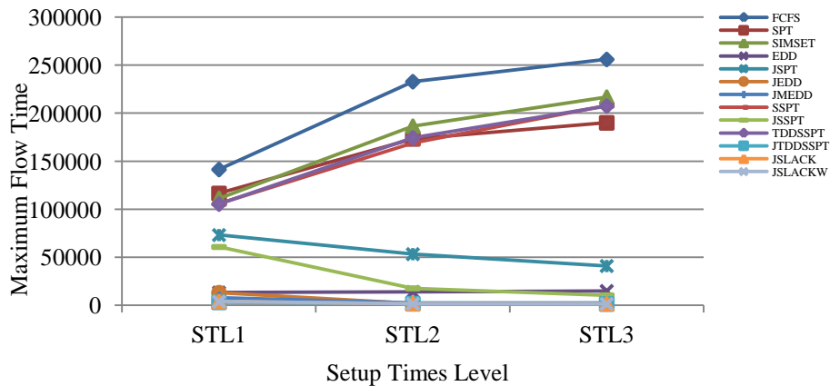
Figure 2. Effect of setup times level on maximum flow time
