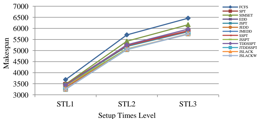
Figure 1. Effect of setup times level on makespan
