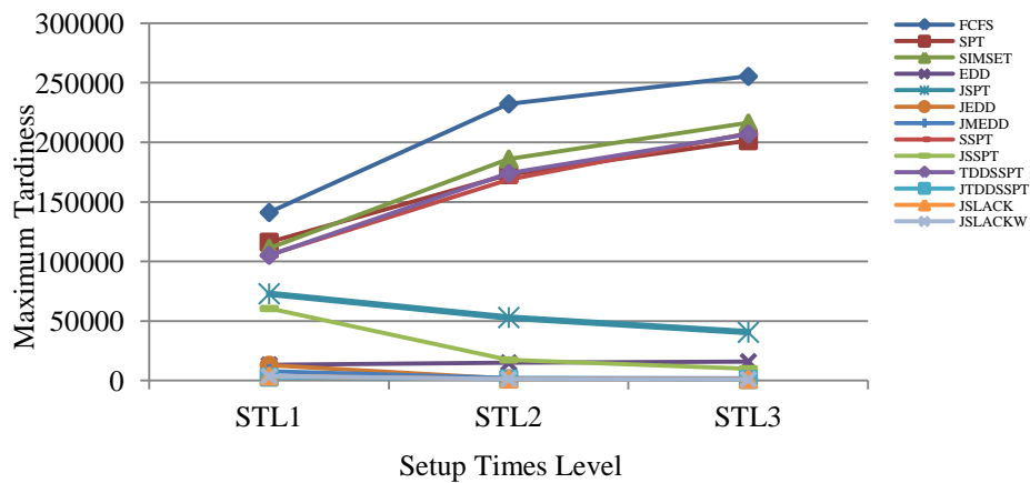
Figure 3. Effect of setup times level on maximum tardiness
