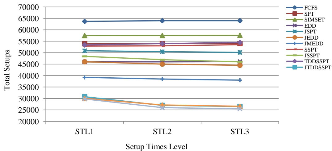
Figure 1. Effect of setup times level on total setups
