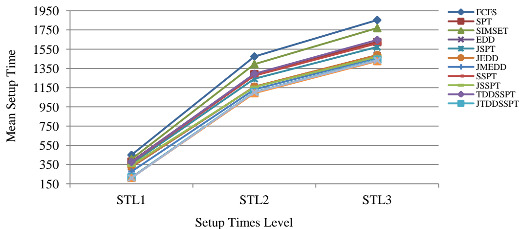
Figure 2. Effect of setup times level on mean setup time
