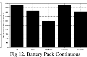
Fig 12. Battery Pack Continuous Current
